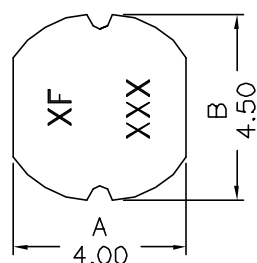
Mechanical Dimensions:
