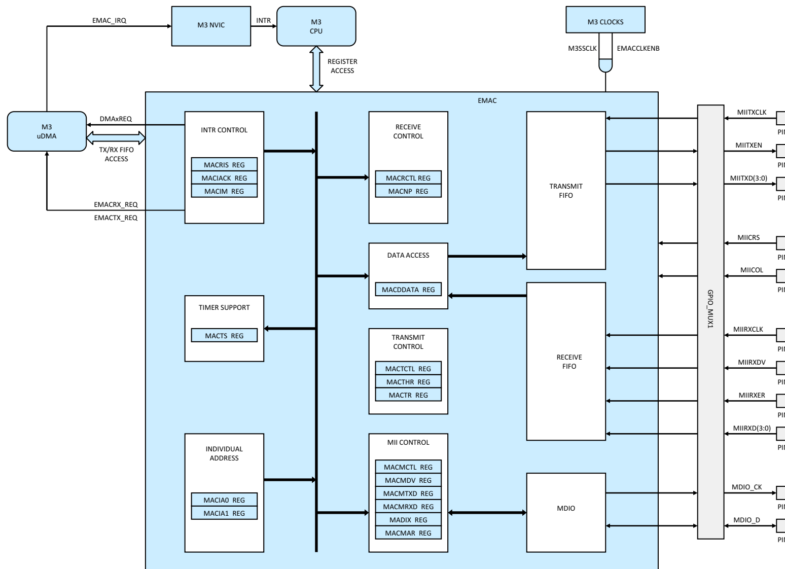
Figure 5-35. EMAC
