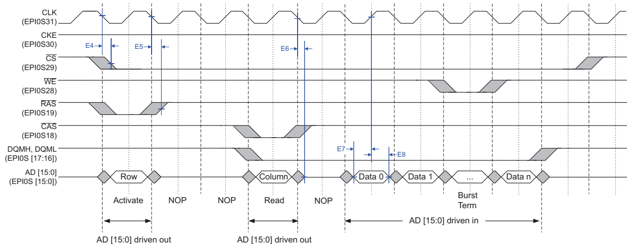
Figure 5-22. SDRAM Read Timing
