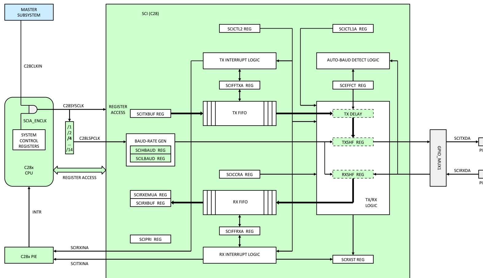
Figure 5-49. SCI (C28x)
