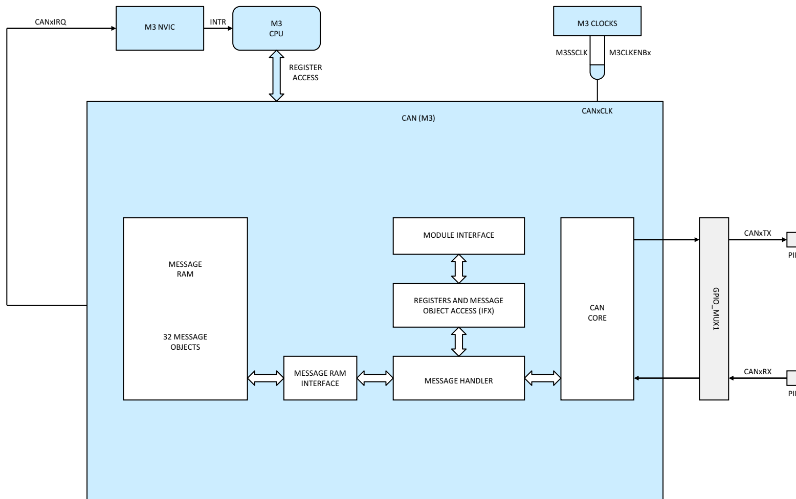
Figure 5-33. CAN (Cortex-M3)
