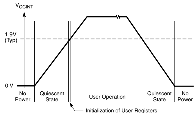
Figure 18: Device Behavior During Power-up
