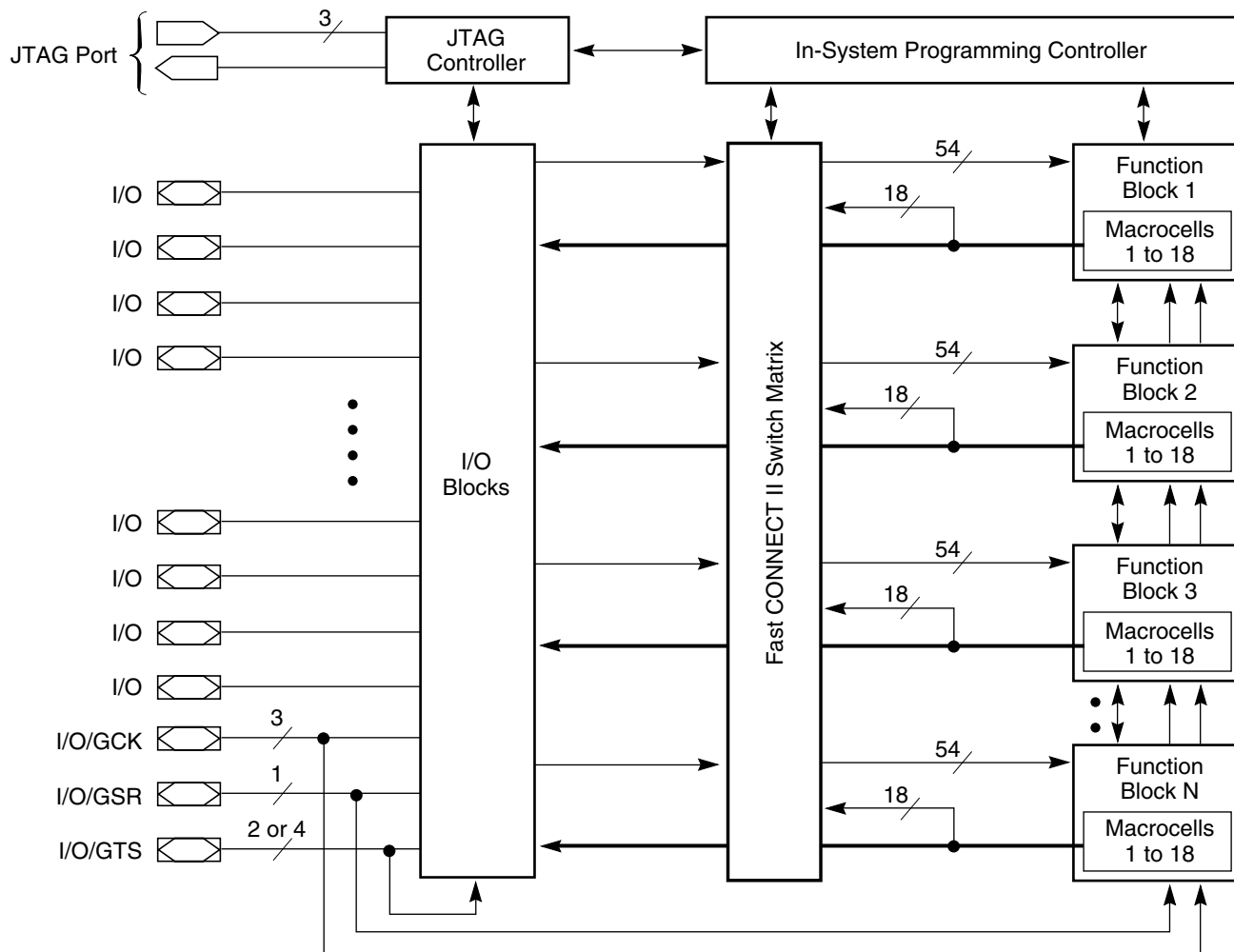
Figure 1: XC9500XV Architecture
