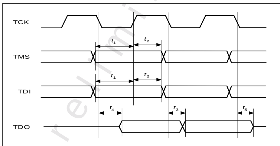
Figure 45 JTAG Timing
