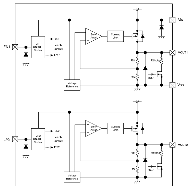
< XC6419BBseries >
