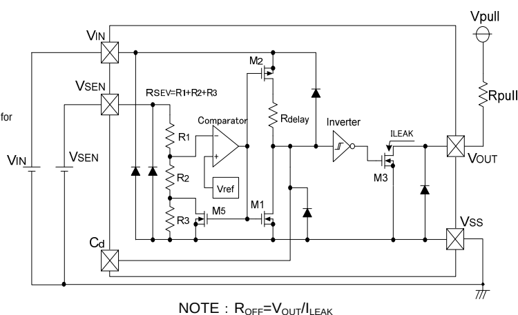
Figure 4: Circuit example of XC6118N Series
