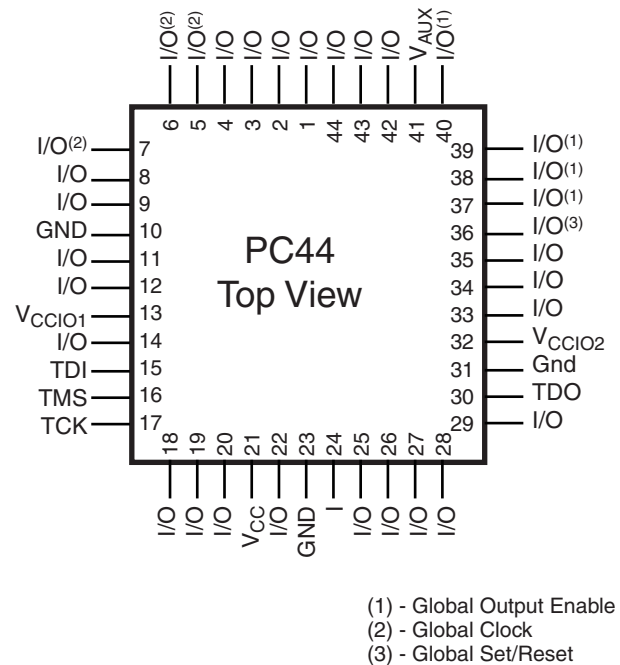
Figure 8: PC44 Package
