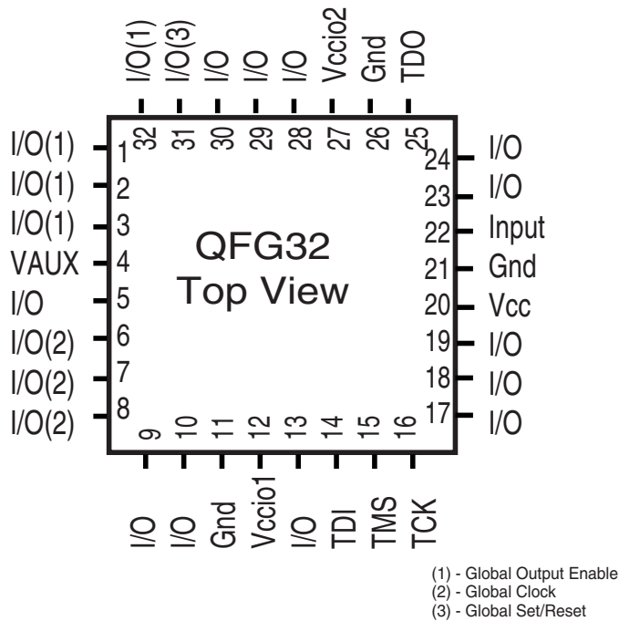
Figure 6: QFG32 Package
