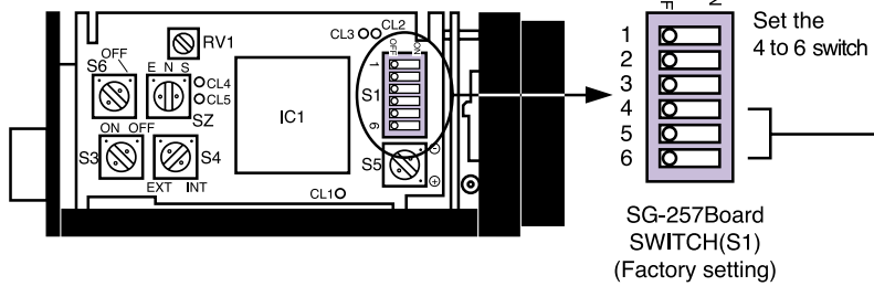
SG-257 Board
