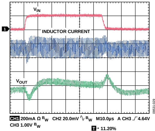
Figure 29. Line Transient, V_{OUT} = 1.8\text{ V} , PWM Mode, 800\text{ mA} , V_{IN} = 4\text{ V} to 5\text{ V} , 2\text{ }\mu\text{s} Rise Time, C_{IN} = 3.3\text{ }\mu\text{F}
