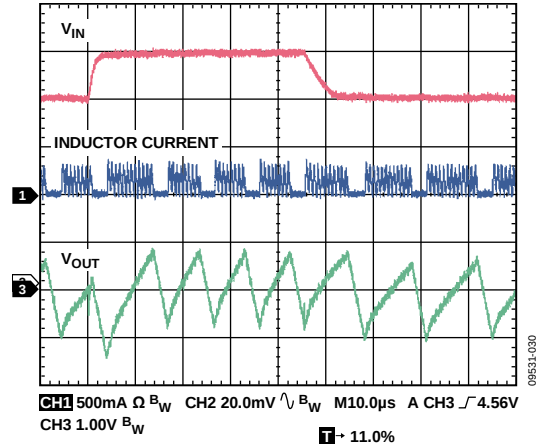
Figure 30. Line Transient, V_{OUT} = 1.2\text{ V} , PSM Mode, 100\text{ mA} , V_{IN} = 4\text{ V} to 5\text{ V} , 2\text{ }\mu\text{s} Rise Time, C_{IN} = 3.3\text{ }\mu\text{F}
