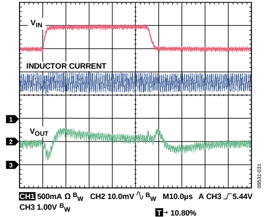
Figure 31. Line Transient, V_{OUT} = 1.2\text{ V} , PWM Mode, 800\text{ mA} , V_{IN} = 4\text{ V} to 5\text{ V} , 2\text{ }\mu\text{s} Rise Time, C_{IN} = 3.3\text{ }\mu\text{F}
