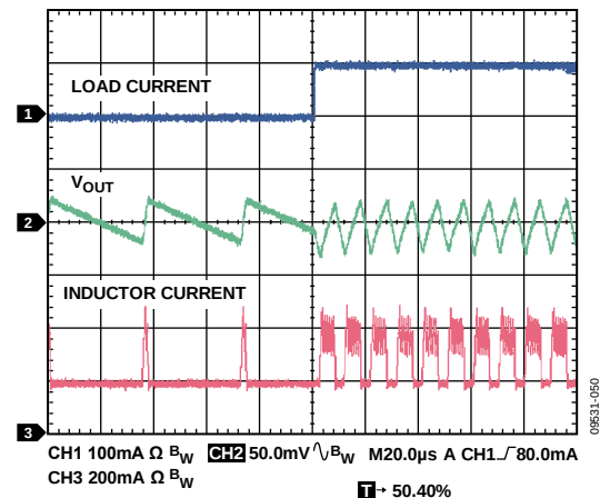
Figure 50. Load Transient, V_{OUT} = 5 V, 10 mA to 110 mA, Load Current Rise Time = 200 ns, V_{IN} = 8 V
