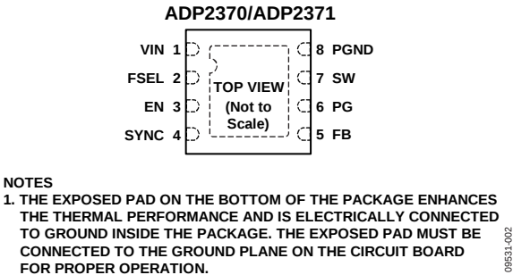
Figure 2. Pin Configuration
