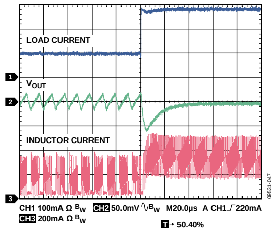
Figure 47. Load Transient, V_{OUT} = 1.2 V, 100 mA to 300 mA, Load Current Rise Time = 200 ns, V_{IN} = 5 V
