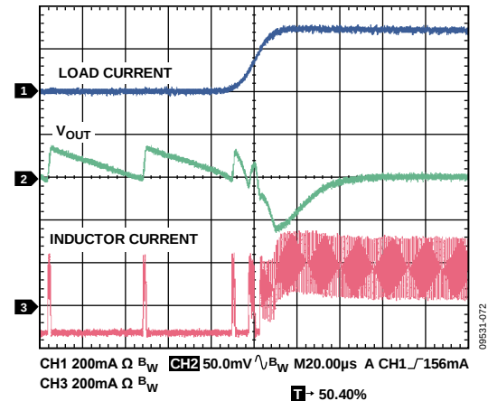
Figure 72. PSM to PWM Transition Waveforms, V_{OUT} = 1.8\text{ V} , 10 mA Load to 300 mA Load
