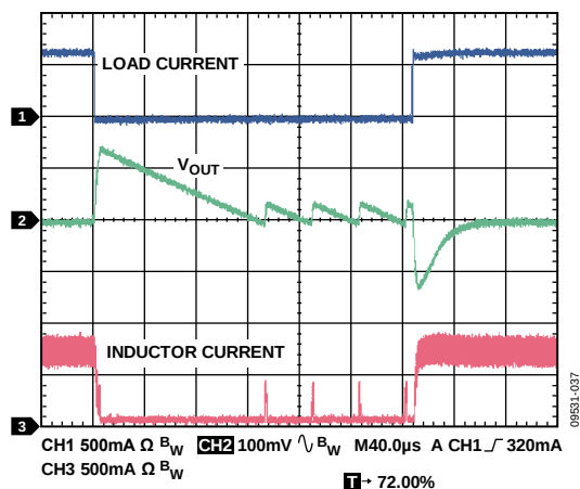
Figure 37. Load Transient, V_{OUT} = 1.8V , 10 mA to 800 mA, Load Current Rise Time = 200 ns
