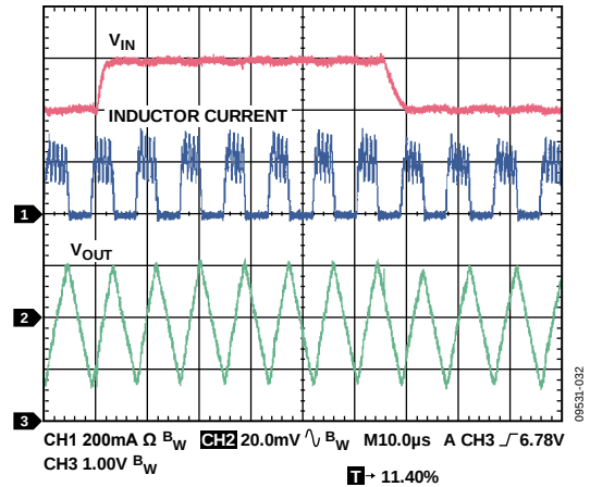
Figure 32. Line Transient, V_{OUT} = 3.3\text{ V} , PSM Mode, 100\text{ mA} , V_{IN} = 6\text{ V} to 7\text{ V} , 2\text{ }\mu\text{s} Rise Time, C_{IN} = 3.3\text{ }\mu\text{F}
