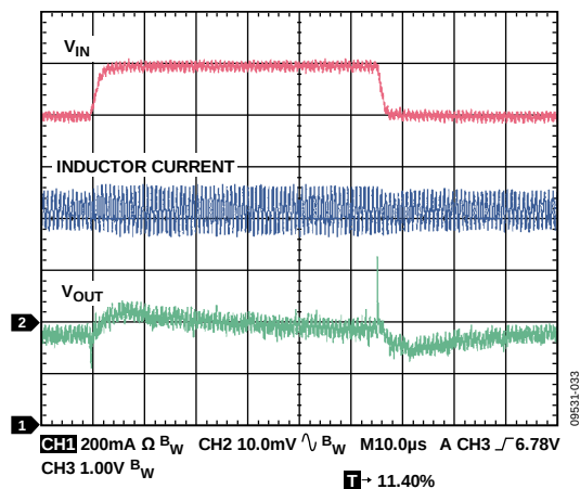
Figure 33. Line Transient, V_{OUT} = 3.3V , PWM Mode, 800 mA, V_{IN1} = 6V to 7V, 2µs Rise Time, C_{IN} = 3.3\mu F
