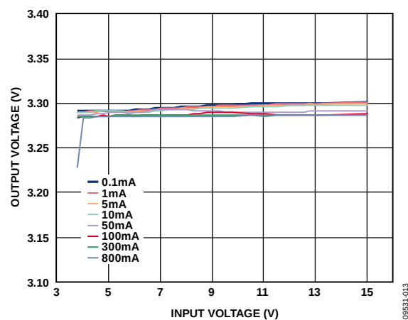
Figure 13. Line Regulation, V_{OUT} = 5.0\text{ V} , Different Loads
