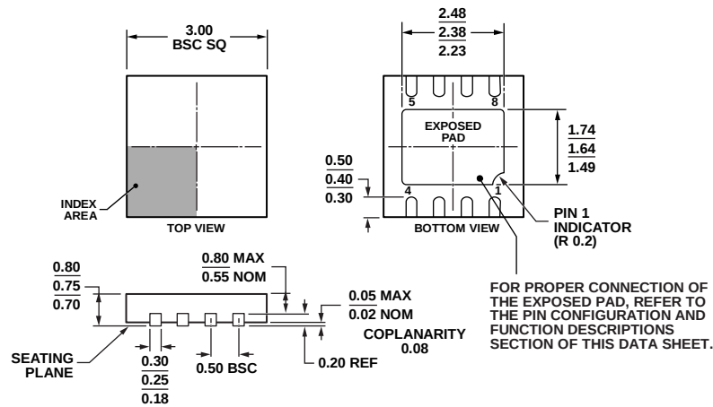
Figure 93. 8-Lead Lead Frame Chip Scale Package [LFCSP] (CP-8-5)
