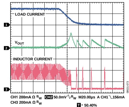
Figure 73. PWM to PSM Transition Waveforms, V_{OUT} = 1.8\text{ V} , 300 mA Load to 10 mA Load
