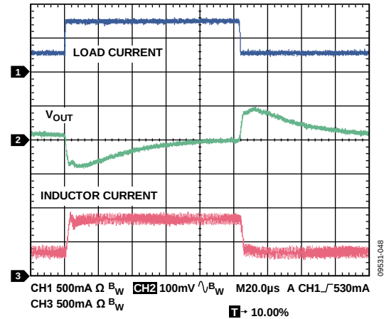
Figure 48. Load Transient, V_{OUT} = 5 V, 300 mA to 800 mA, Load Current Rise Time = 200 ns, V_{IN} = 8 V
