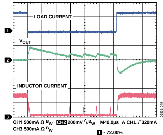
Figure 49. Load Transient, V_{OUT} = 5 V, 1 mA to 800 mA, Load Current Rise Time = 200 ns, V_{IN} = 8 V
