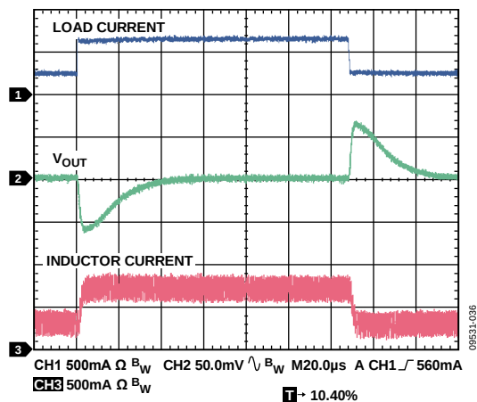
Figure 36. Load Transient, V_{OUT} = 1.8V , 300 mA to 800 mA, Load Current Rise Time = 200 ns
