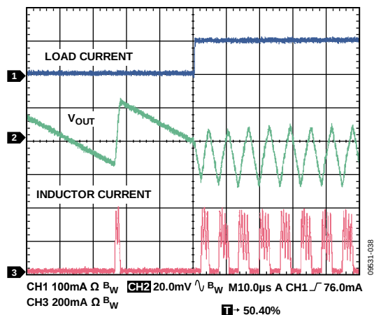
Figure 38. Load Transient, V_{OUT} = 1.8V , 10 mA to 110 mA, Load Current Rise Time = 200 ns
