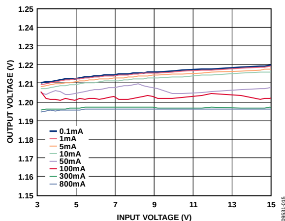
Figure 15. Line Regulation, V_{OUT} = 1.2\text{ V} , Different Loads
