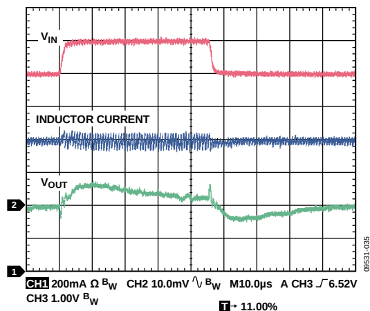
Figure 35. Line Transient, V_{OUT} = 5V , PWM Mode, 800 mA, V_{IN1} = 6V to 7V, 2µs Rise Time, C_{IN} = 3.3\mu F
