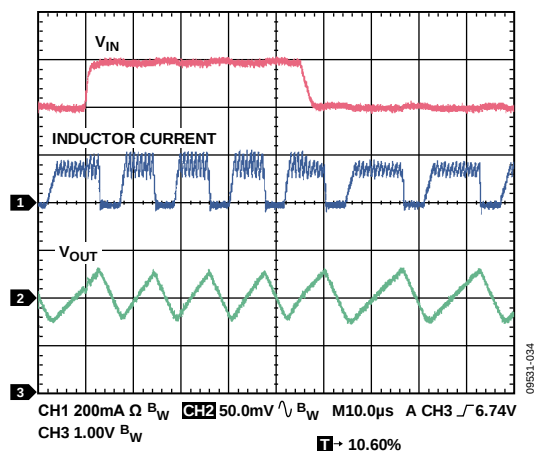
Figure 34. Line Transient, V_{OUT} = 5V , PSM Mode, 100 mA, V_{IN1} = 6V to 7V, 2µs Rise Time, C_{IN} = 3.3\mu F
