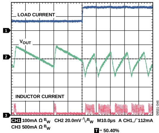
Figure 46. Load Transient, V_{OUT} = 1.2 V, 10 mA to 110 mA, Load Current Rise Time = 200 ns, V_{IN} = 5 V
