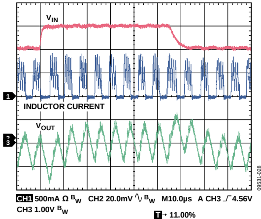
Figure 28. Line Transient, V_{OUT} = 1.8\text{ V} , PSM Mode, 100\text{ mA} , V_{IN} = 4\text{ V} to 5\text{ V} , 2\text{ }\mu\text{s} Rise Time, C_{IN} = 3.3\text{ }\mu\text{F}
