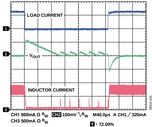
Figure 45. Load Transient, V_{OUT} = 1.2 V, 10 mA to 800 mA, Load Current Rise Time = 200 ns, V_{IN} = 5 V
