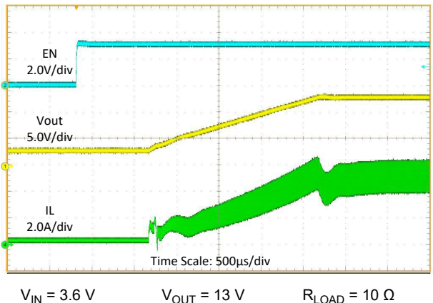
Figure 8-5. Start-up Waveforms
