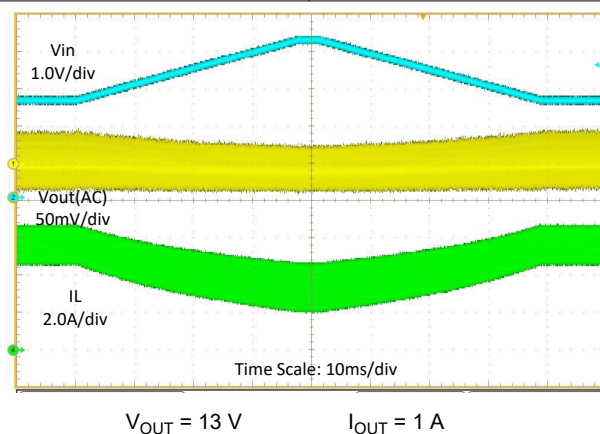
Figure 8-10. Line Sweep ( V_{IN} = 2.7 \text{ V} to 4.2 \text{ V} )
