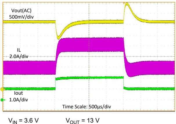
Figure 8-7. Load Transient (I OUT = 1 to 2 A)
