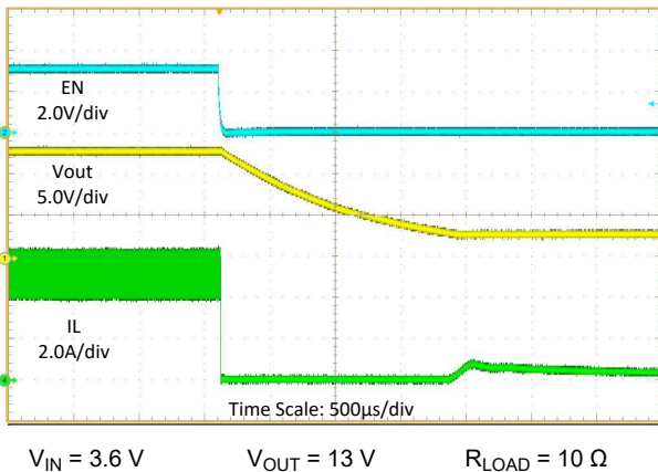
Figure 8-6. Shutdown Waveforms
