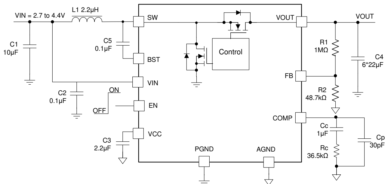
Figure 8-1. TPS61288 3.6-V to 13-V/2.3-A Output Converter
