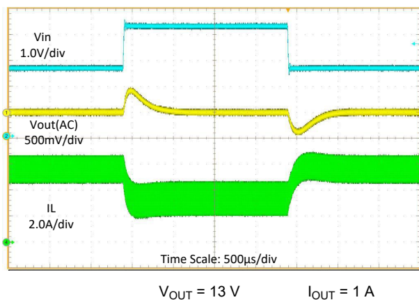
Figure 8-8. Line Transient ( V_{IN} = 2.7 \text{ V} to 4.2 \text{ V} )
