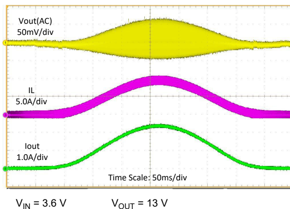
Figure 8-9. Load Sweep ( I_{OUT} = 0 to 2 \text{ A} )
