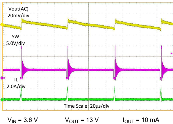
Figure 8-4. Switching Waveforms in 10 mA load
