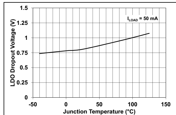
FIGURE 2-6: LDO Regulator Dropout Voltage vs. Temperature.
