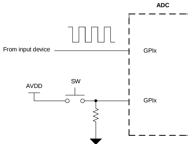
Figure 131. Digital Input
