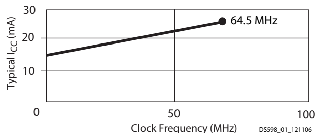
Figure 1: Typical I_{CC} vs. Frequency for XA9536XL
