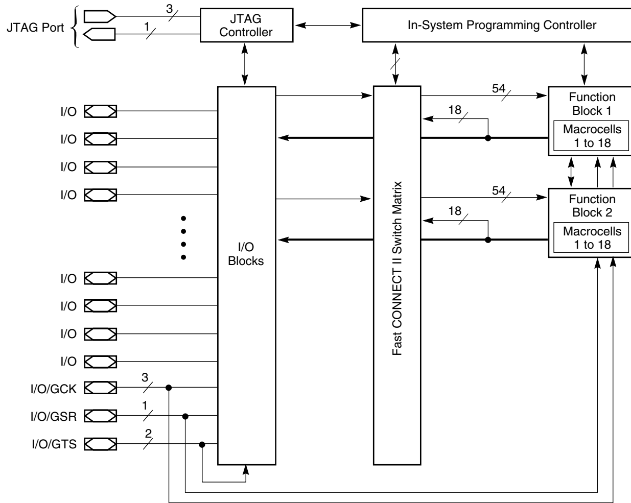
Figure 2: XA9536XL Architecture
