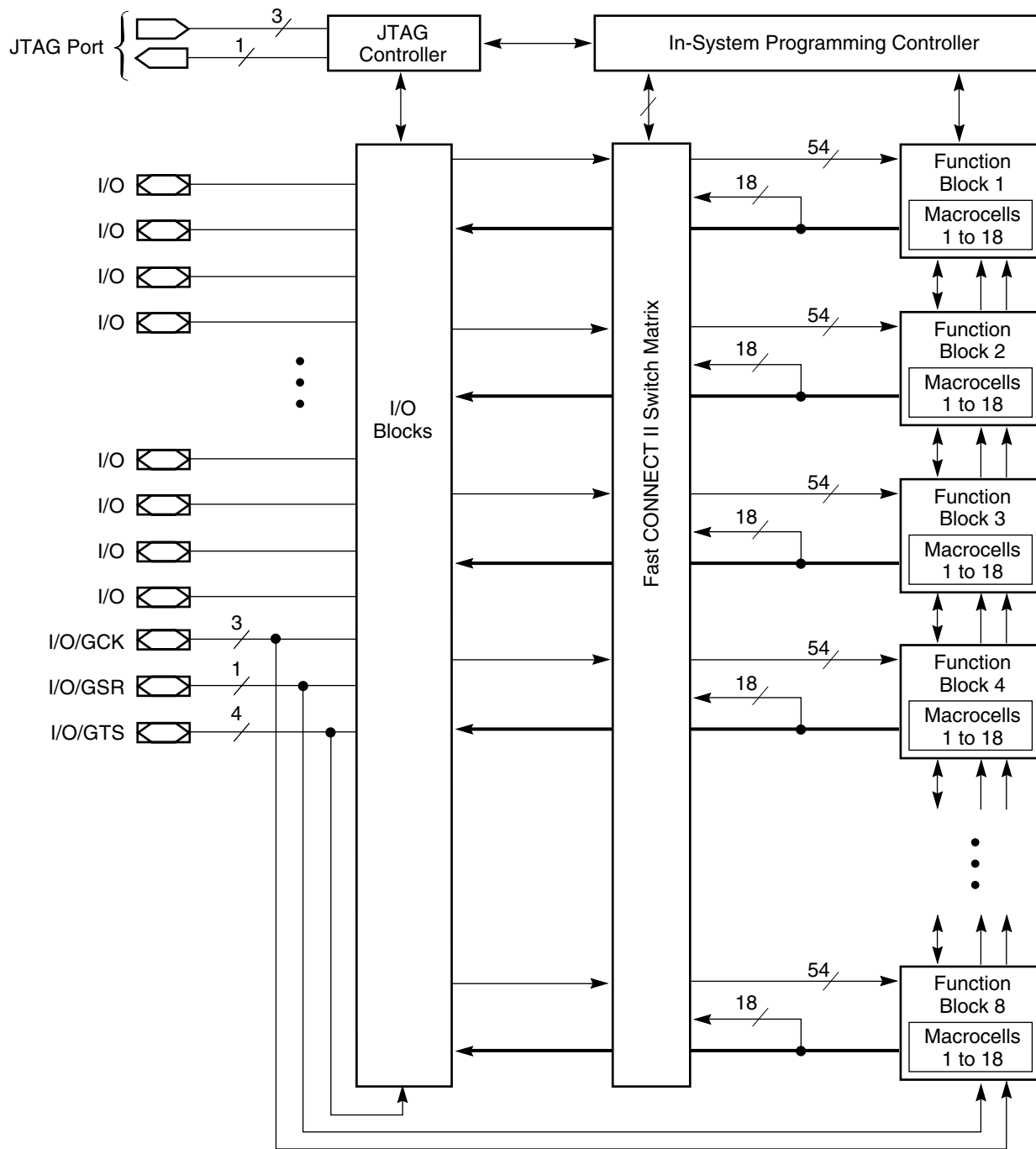
Figure 2: XA95144XL Architecture
