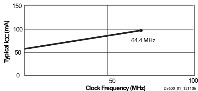
Figure 1: Typical I_{CC} vs. Frequency for XA95144XL
