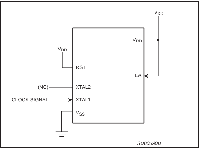
Figure 30. I_{DD} Test Condition, Idle Mode
