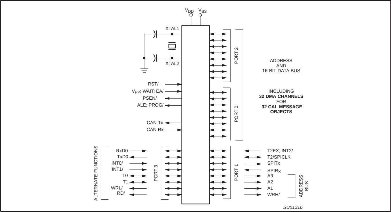
Figure 3. Logic Symbol
