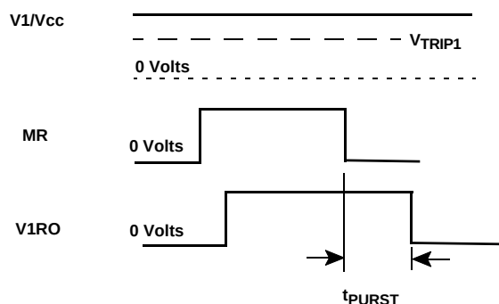
FIGURE 20. MANUAL RESET RESPONSE
