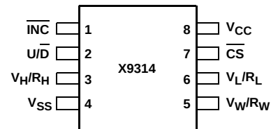
X9314 8 LD SOIC TOP VIEW
