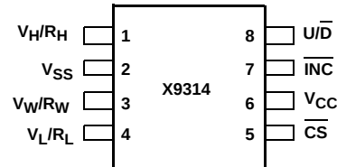
X9314 8 LD MSOP TOP VIEW
