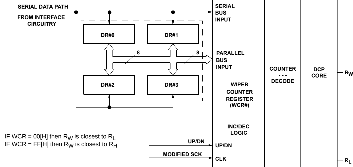
FIGURE 1. DETAILED POTENTIOMETER BLOCK DIAGRAM
