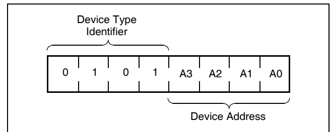
Figure 1. Slave Address
