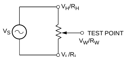
Test Circuit #1
