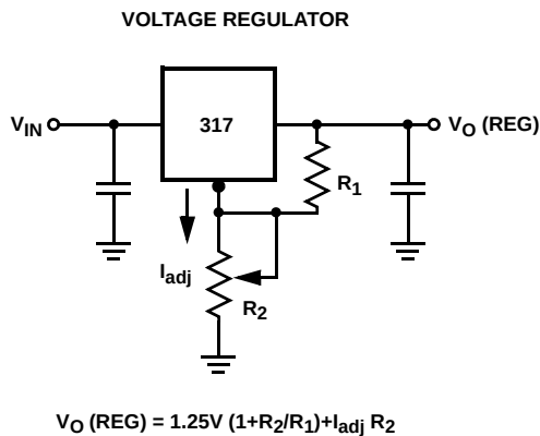
VOLTAGE REGULATOR
