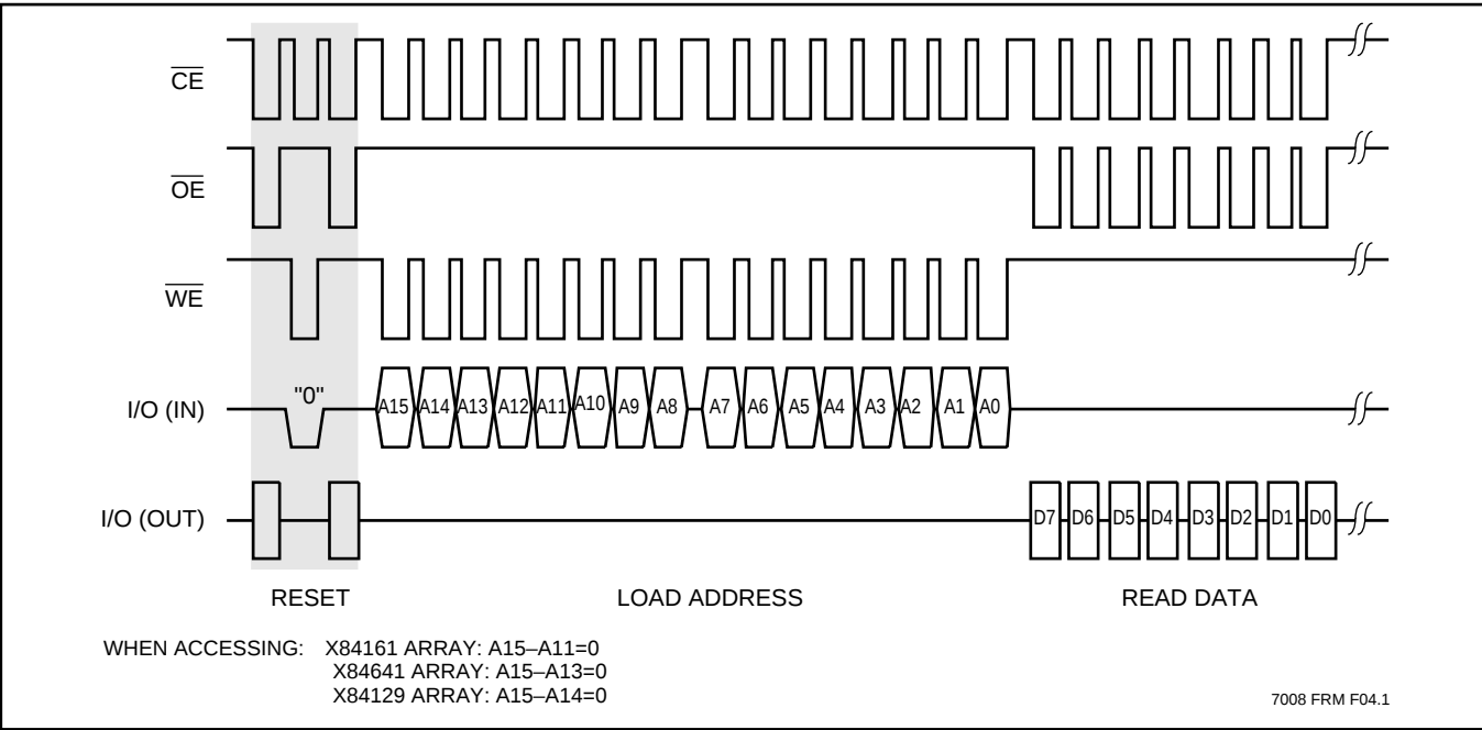
Figure 1. Read Sequence
