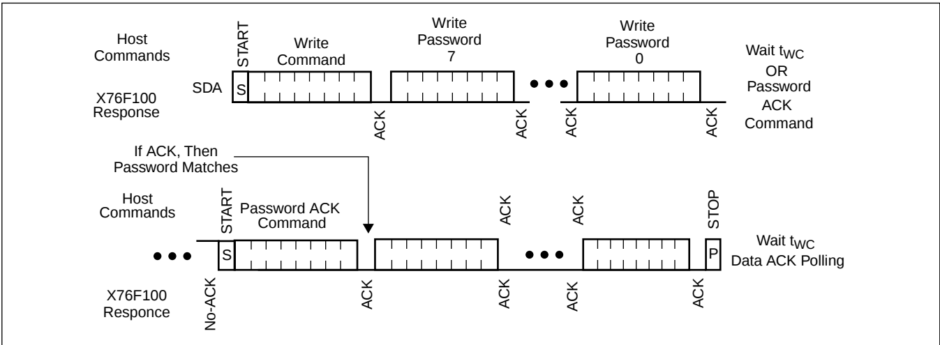
Figure 5. Acknowledge Polling
