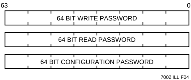
Figure 2. Password Registers
