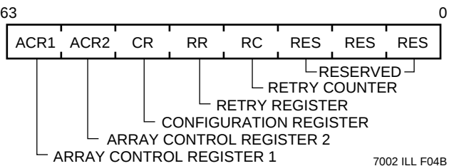
Figure 3. Configuration Registers
