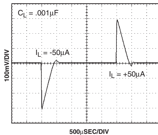
50 \mu A LOAD TRANSIENT RESPONSE
