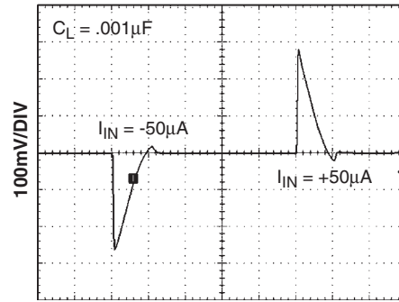
50μA LOAD TRANSIENT RESPONSE
