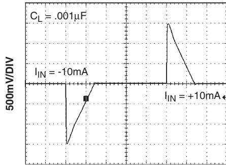
10mA LOAD TRANSIENT RESPONSE
