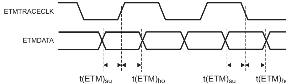
Figure 7-20. ETMDATA Timing
