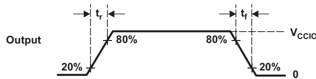
Figure 7-7. CMOS-Level Outputs
