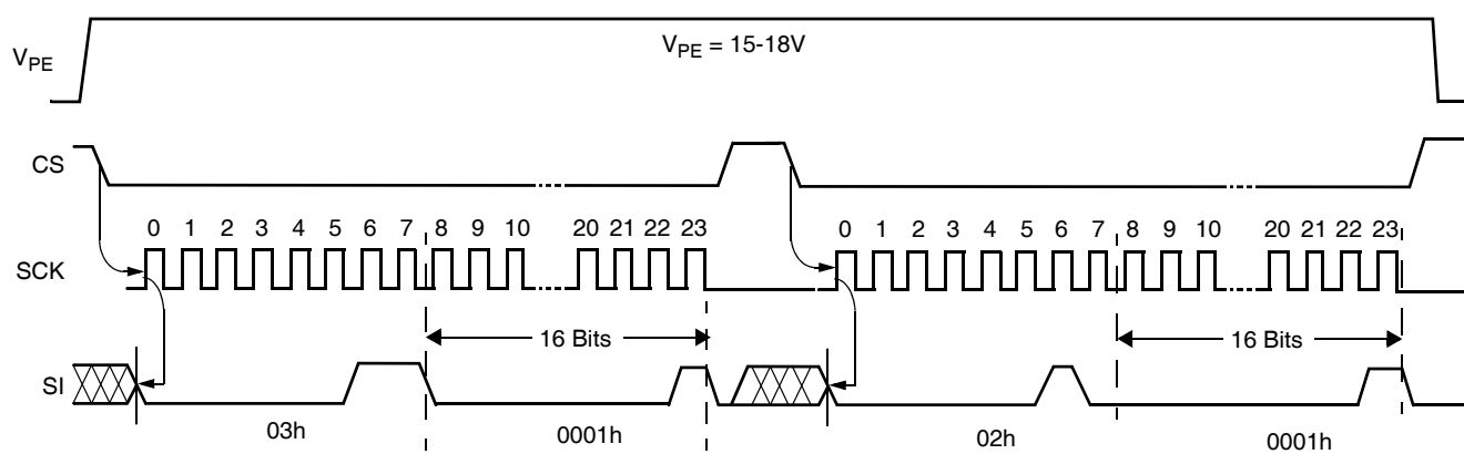
Figure 2. Set V_{TRIP} Level Sequence ( V_{CC} = \text{desired } V_{TRIP} \text{ value} )
