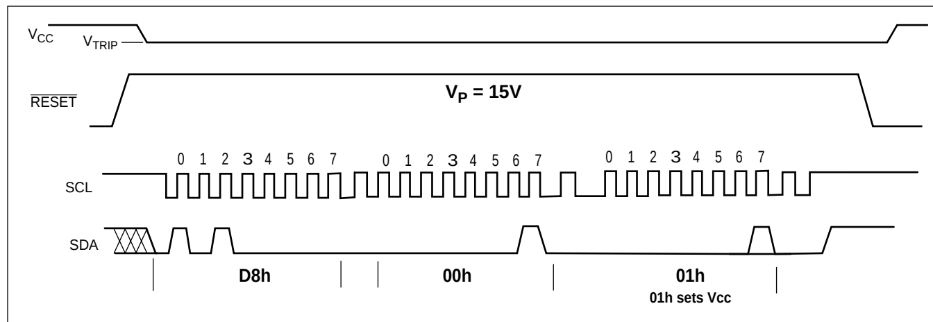
Figure 2. Set V_{TRIP} Level Sequence ( V_{CC} \geq V_{TRIP} )
