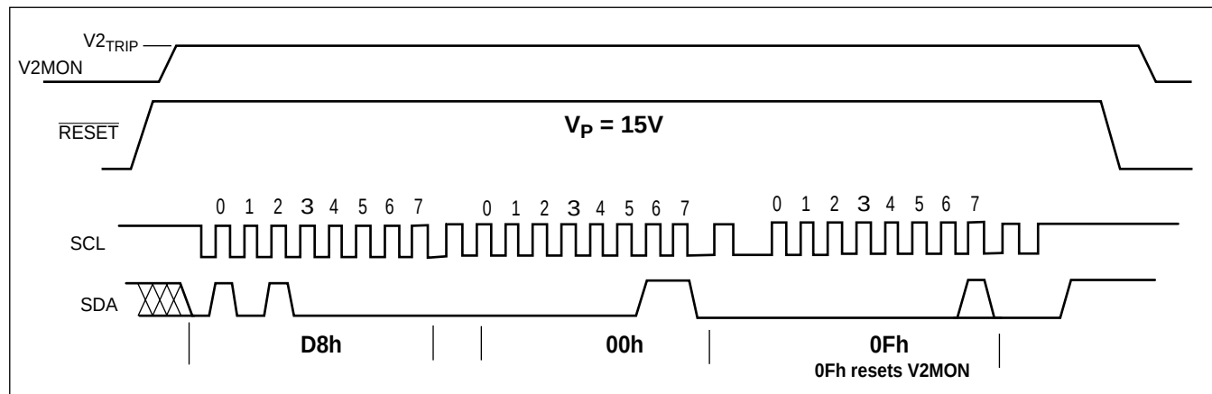
Figure 5. Reset V2 TRIP Level Sequence (V CC > 3V, WEL is set.)
