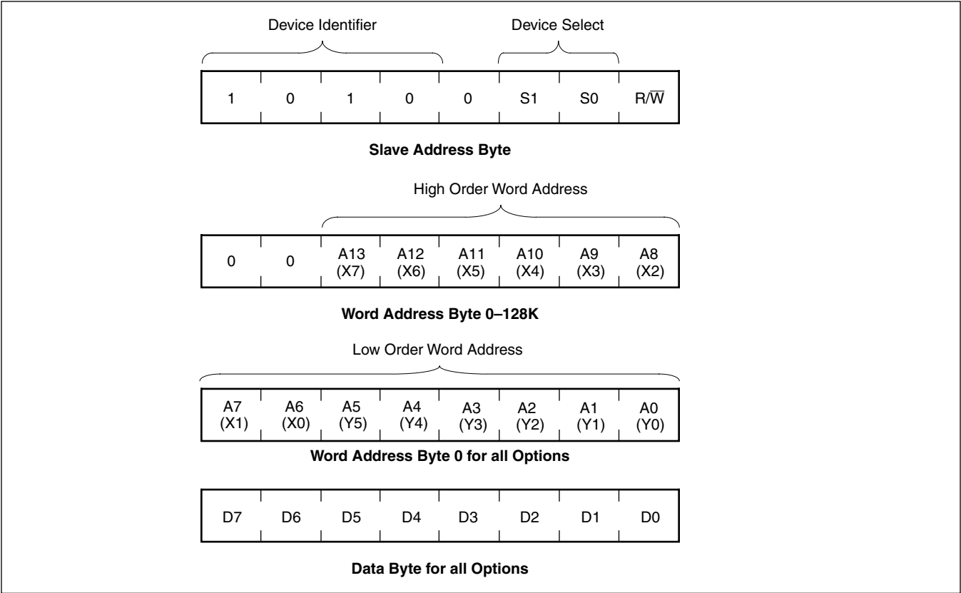
Figure 15. X4283/85 Addressing
