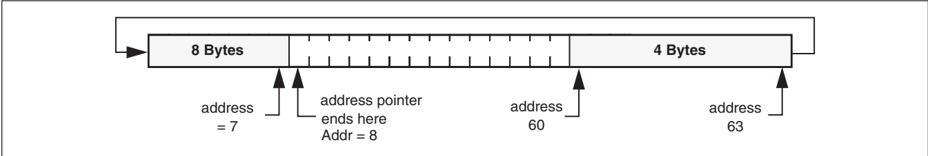
Figure 10. Writing 12 bytes to a 64-byte page starting at location 60 (Wrap around).
