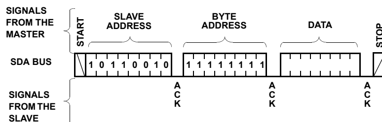
FIGURE 9. WRITE CONTROL REGISTER SEQUENCE
