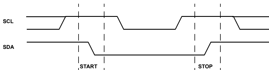
FIGURE 7. VALID START AND STOP CONDITIONS
