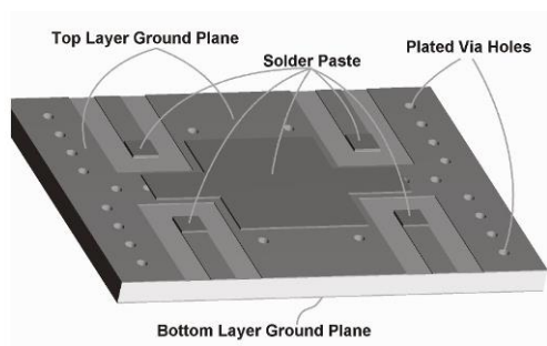
Figure 2: Solder Paste Application
