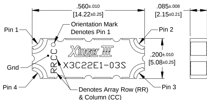
Dimensions Are in Inches [Millimeters] X3C22E1-03S Mechanical Outline
