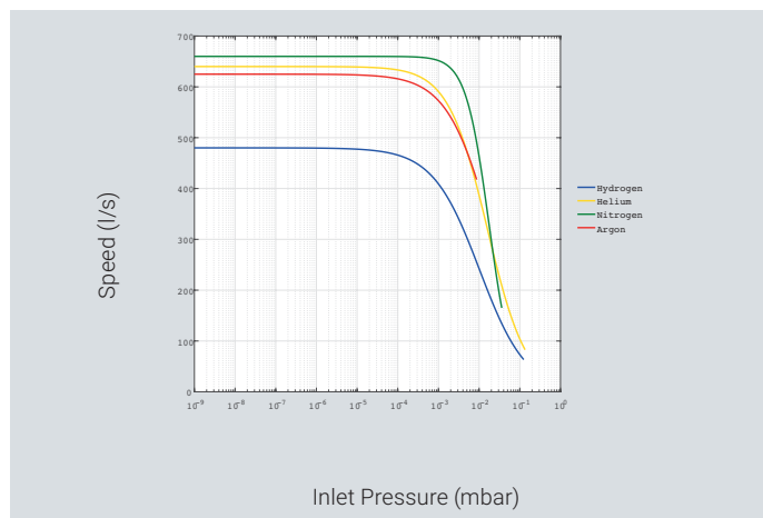
Pumping Speed
