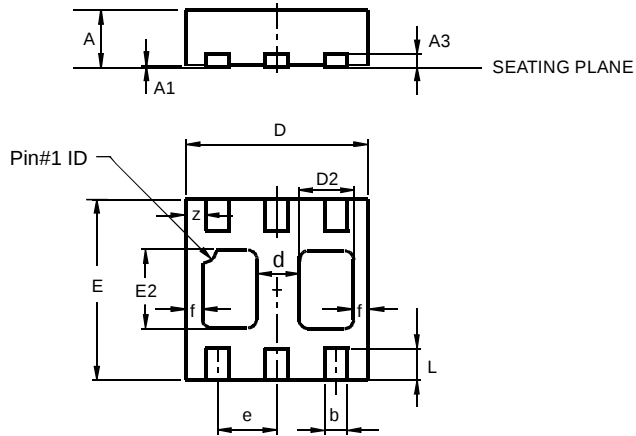
U-DFN2020-6 Type B
