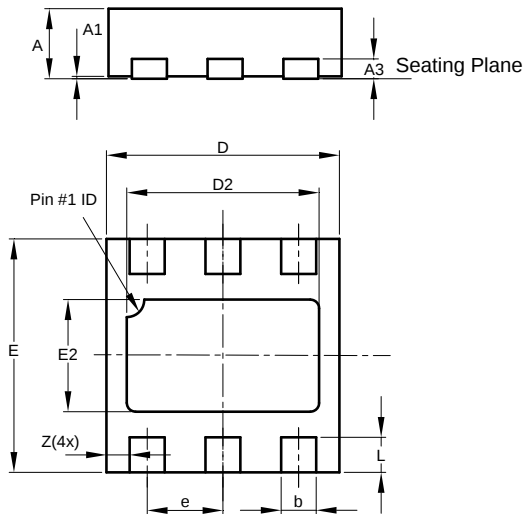
U-DFN2020-6 Type C
