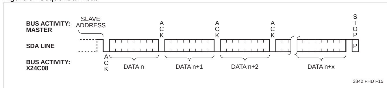
Figure 9. Sequential Read
