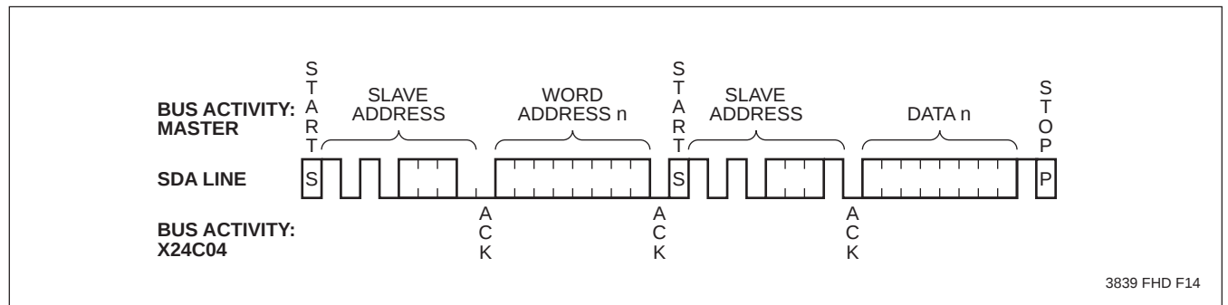
Figure 8. Random Read
