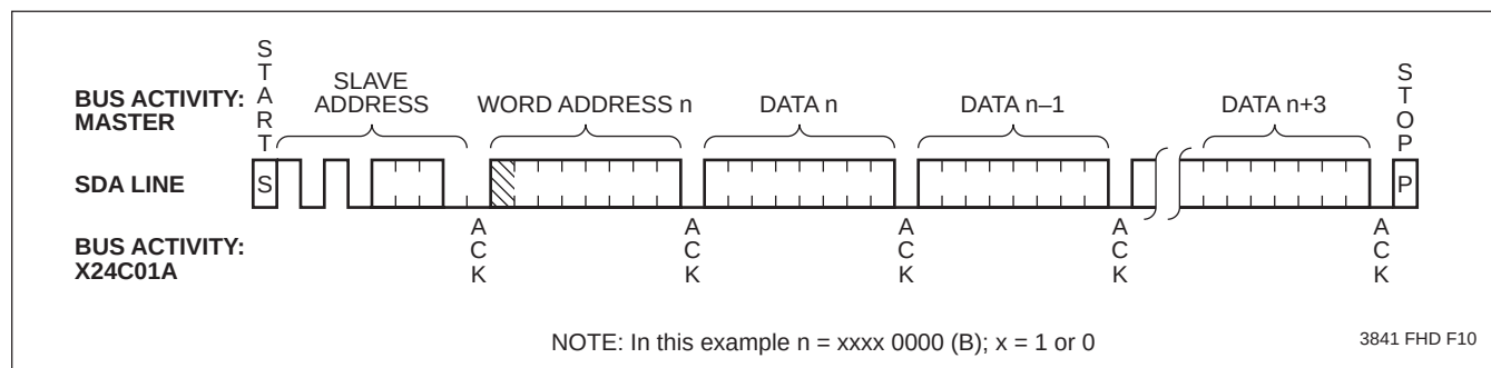
Figure 6. Page Write
