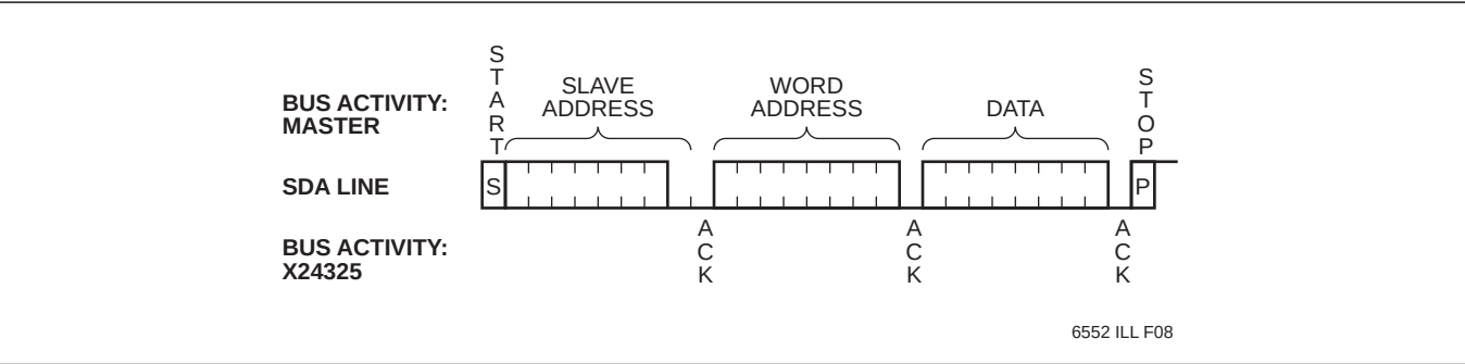
Figure 5. Byte Write
