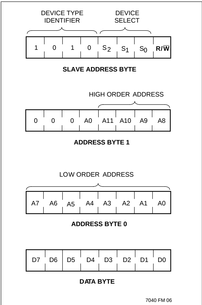
Figure 4. Device Addressing
