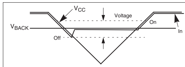
Figure 2. Power Control
