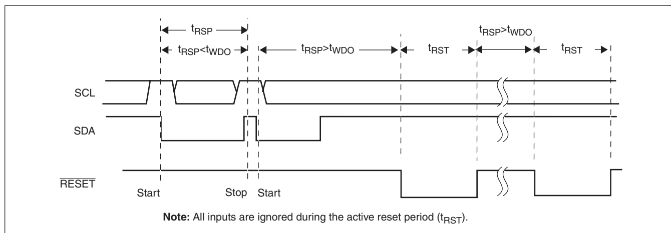
Figure 3. Watchdog Restart/Time Out
