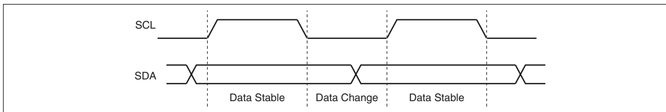
Figure 8. Valid Start and Stop Conditions
