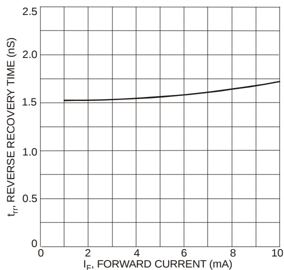
Fig. 6 Typical Reverse Recovery Time vs. Forward Current
