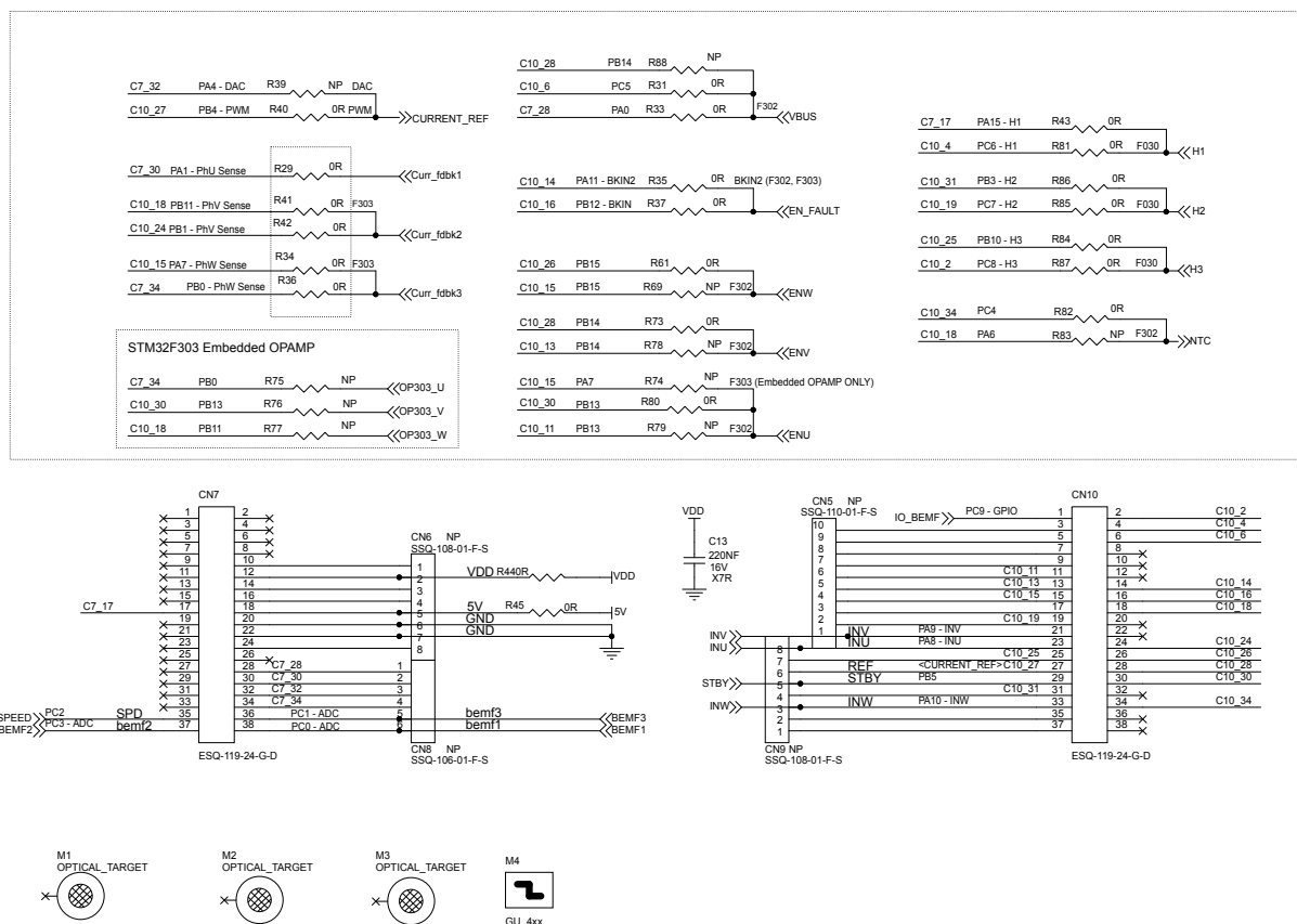
Figure 4. X-NUCLEO-IHM16M1 circuit schematic (4 of 5)
