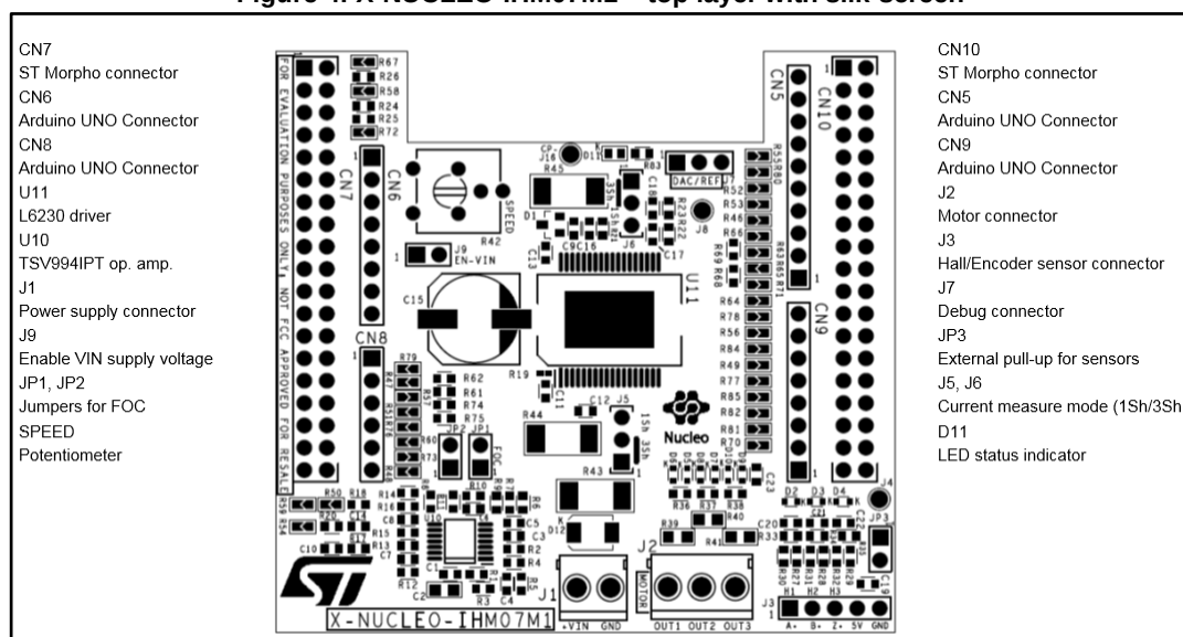
Figure 4: X-NUCLEO-IHM07M1 – top layer with silk-screen
