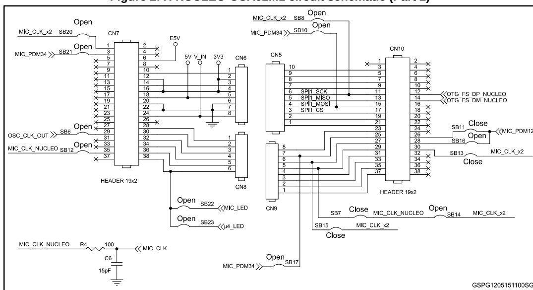
Figure 2: X-NUCLEO-CCA02M1 circuit schematic (Part 2)
