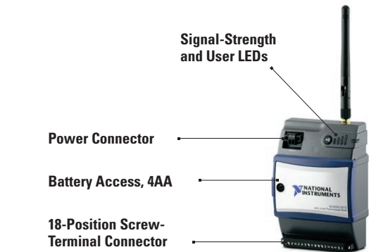
Figure 6. Measurement Node External Features
