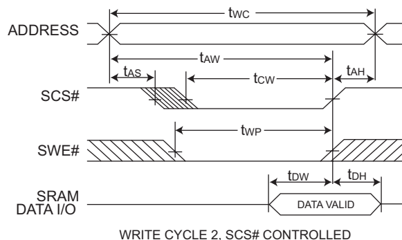
FIGURE 6 – SRAM WRITE CYCLE SCS# CONTROLLED
