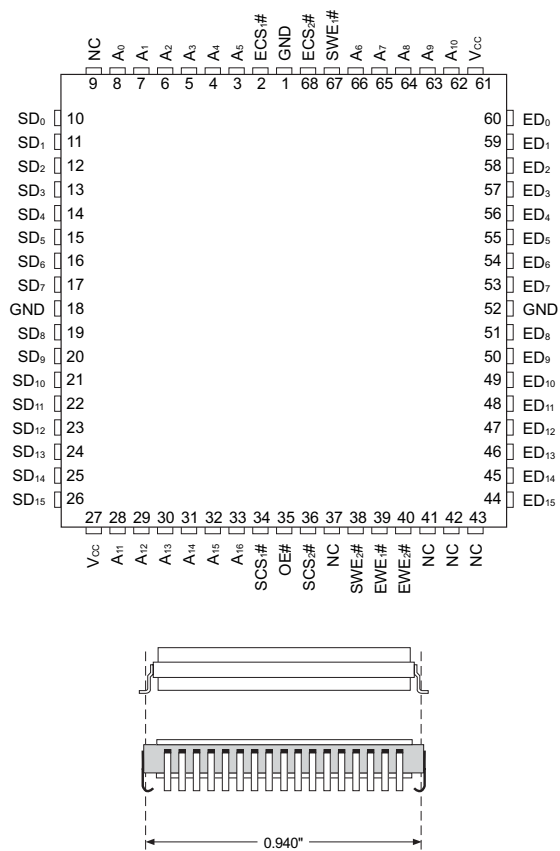
FIGURE 2 WSE128K16-XG2TX PIN CONFIGURATION
