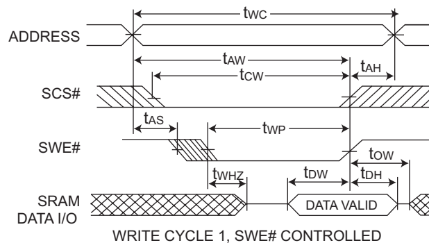
FIGURE 5 – SRAM WRITE CYCLE SWE# CONTROLLED
