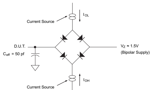
FIGURE 3 – AC TEST CIRCUIT
