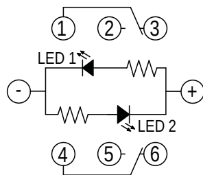
DPDT
