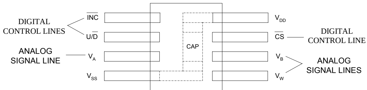
FIGURE 9 – WMS7110/1 LAYOUT
