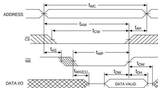
WRITE CYCLE 1 \overline{WE} CONTROLLED ( \overline{OE} = V_{IH} )
